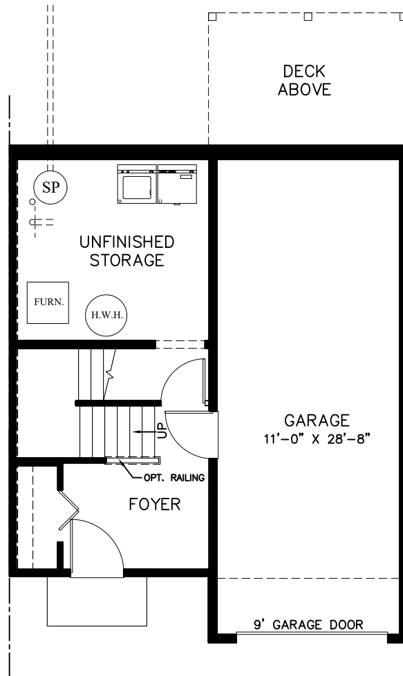
FOUNDATION DIAGRAM
